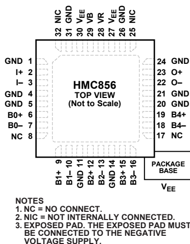
Figure 3. Pin Configuration
