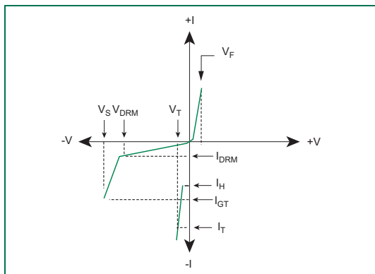
V-I Characteristics
