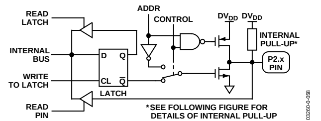
Figure 59. Port 2 Bit Latch and I/O Buffer
