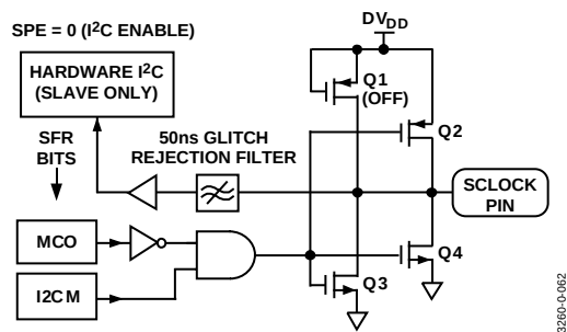
Figure 63. SCLOCK Pin I/O Functional Equivalent in I²C Mode
