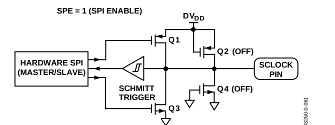
Figure 62. SCLOCK Pin I/O Functional Equivalent in SPI Mode
