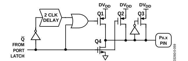
Figure 60. Internal Pull-Up Configuration
