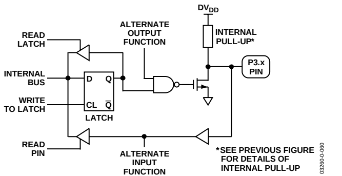
Figure 61. Port 3 Bit Latch and I/O Buffer
