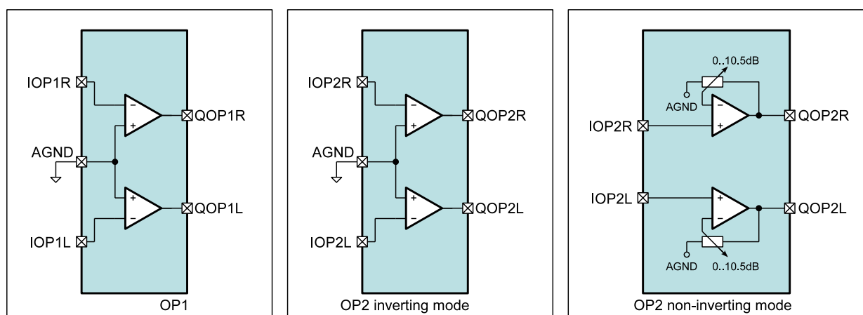
Figure 14. Operational Amplifiers
