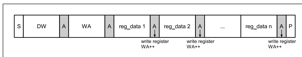
Figure 20. Page Write
