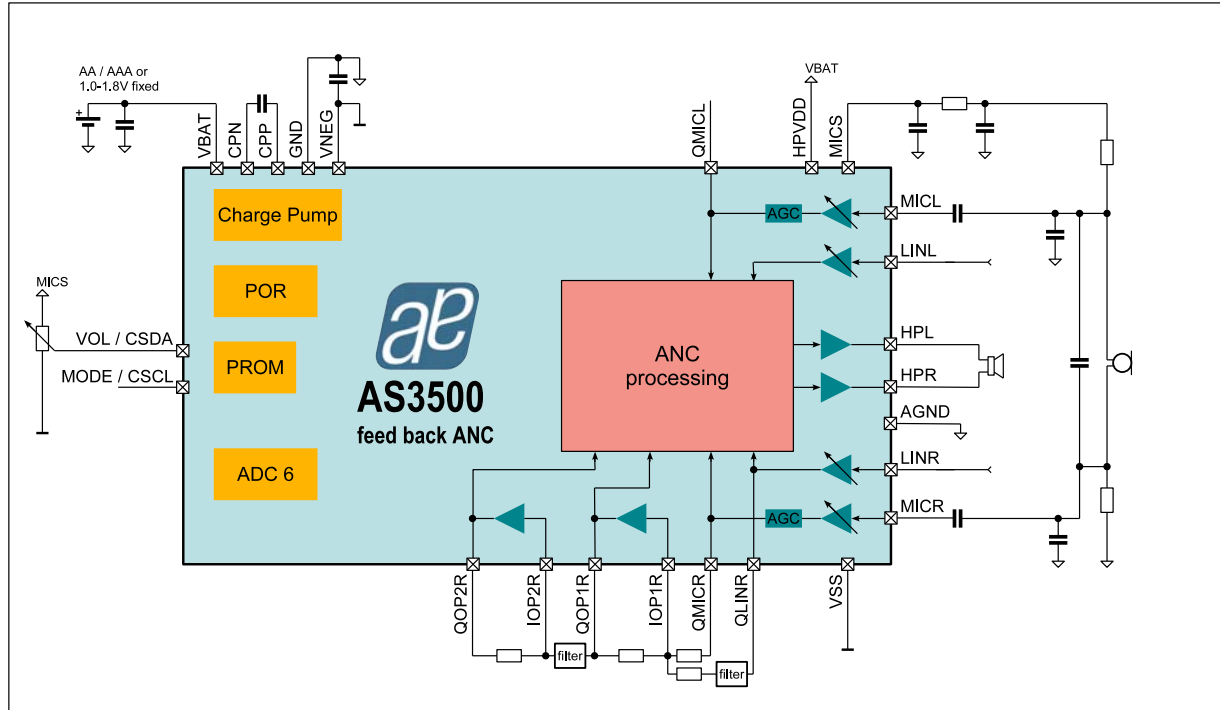
Figure 3. AS3500 Feed-Forward Block Diagram
