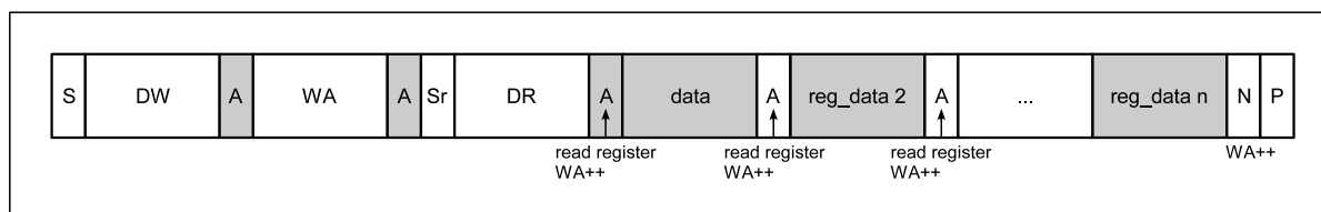
Figure 22. Sequential Read
