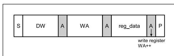
Figure 19. Byte Write
