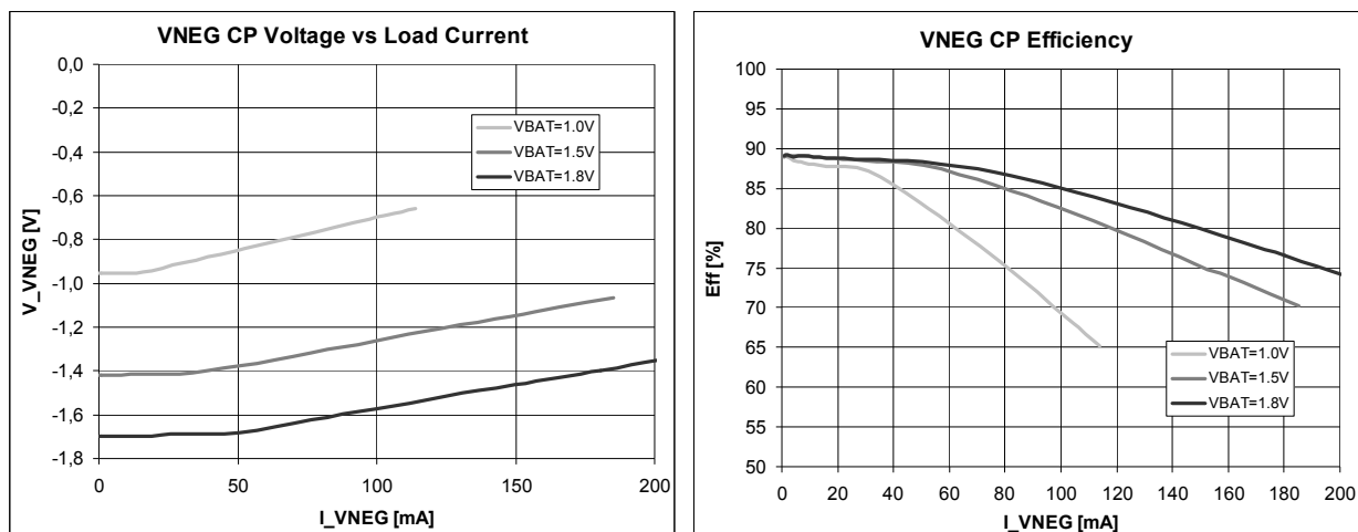
Figure 6. VNEG Charge Pump
