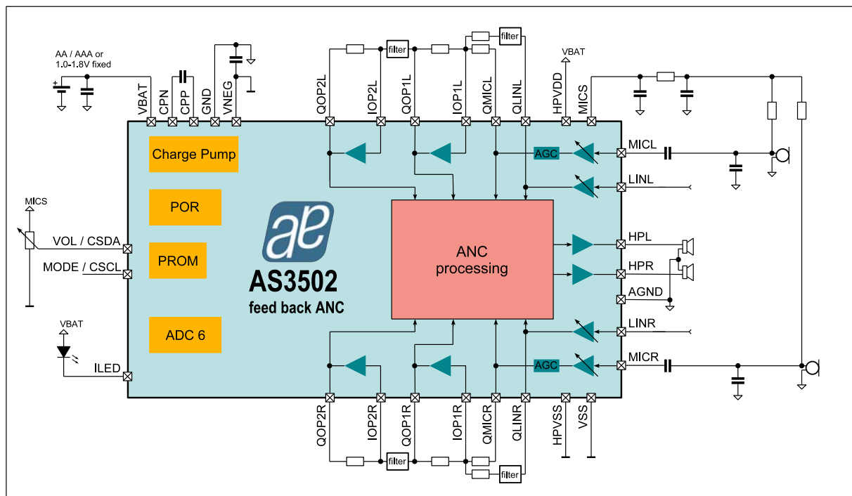
Figure 2. AS3502 Feed-Back Block Diagram
