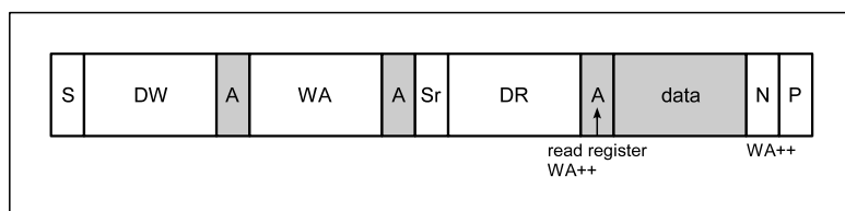
Figure 21. Random Read
