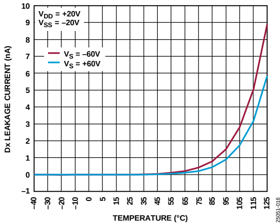
Figure 15. Dx Leakage Current vs. Temperature During Overvoltage, \pm 20 V Dual Supply
