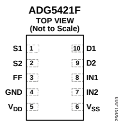
Figure 2. Pin Configuration
