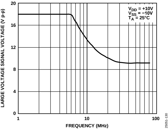
Figure 30. Large Voltage Signal Voltage vs. Frequency
