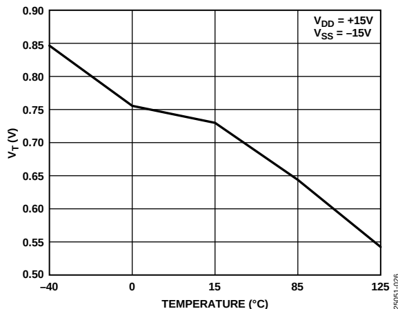
Figure 25. V_T vs. Temperature, ±15 V Dual Supply
