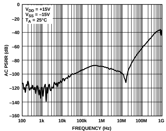
Figure 20. AC Power Supply Rejection Ratio (PSRR) vs. Frequency, \pm 15 V Dual Supply
