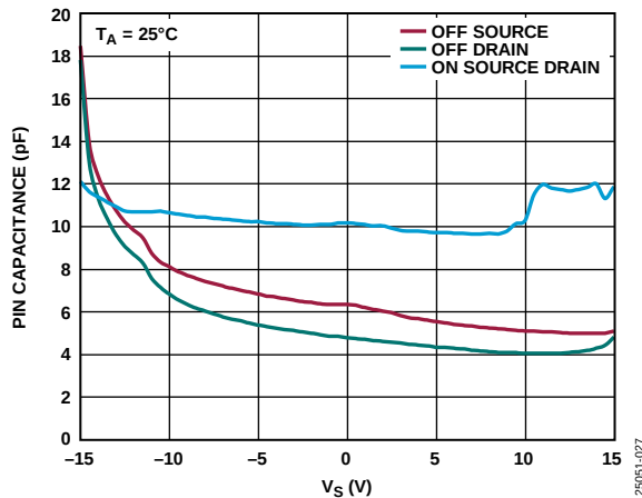
Figure 26. Pin Capacitance vs. V_S
