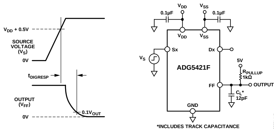
Figure 43. Interrupt Flag Response Time, t_{\text{DIGRESP}} ( V_{\text{FF}} Is the Fault Flag Voltage)
