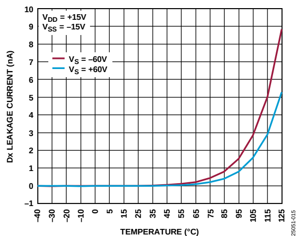
Figure 14. Dx Leakage Current vs. Temperature During Overvoltage, ±15 V Dual Supply
