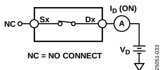
Figure 33. On Leakage
