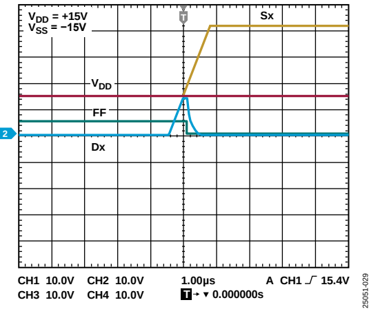
Figure 28. Drain Output Response to Positive Overvoltage
