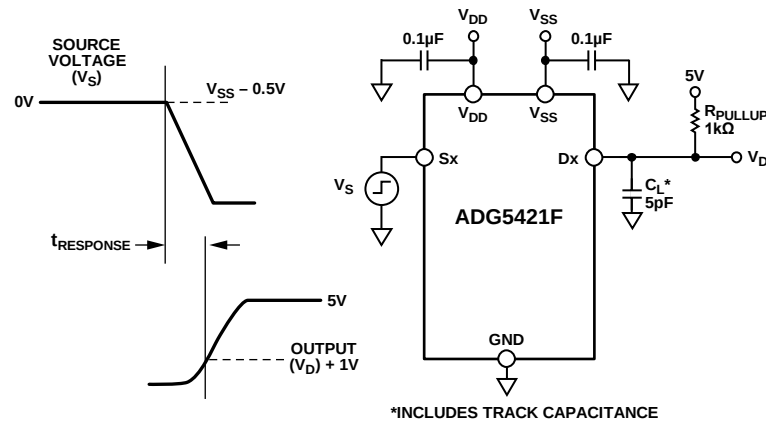
Figure 41. Negative Overvoltage Response Time, Single-Supply, t_{\text{RESPONSE}}
