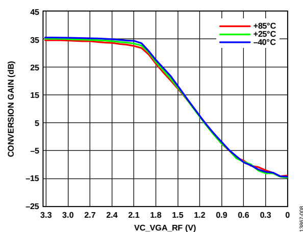
Figure 8. Conversion Gain vs. VC\_VGA\_RF at RF = 2\text{ GHz} , 56 MHz Filter ( RF\text{ Input Power} = -40\text{ dBm} , VC\_VGA\_IF = 0\text{ V} )
