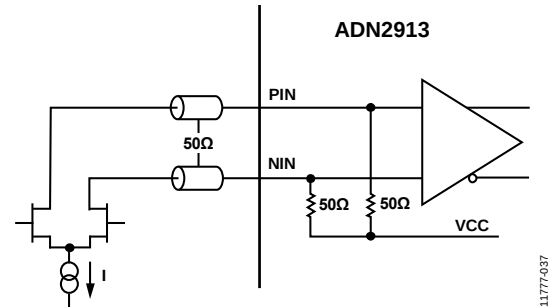
Figure 36. DC-Coupled Application, 0 dB EQ Input (Normal Mode)
