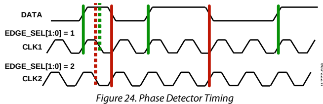
Figure 24. Phase Detector Timing
