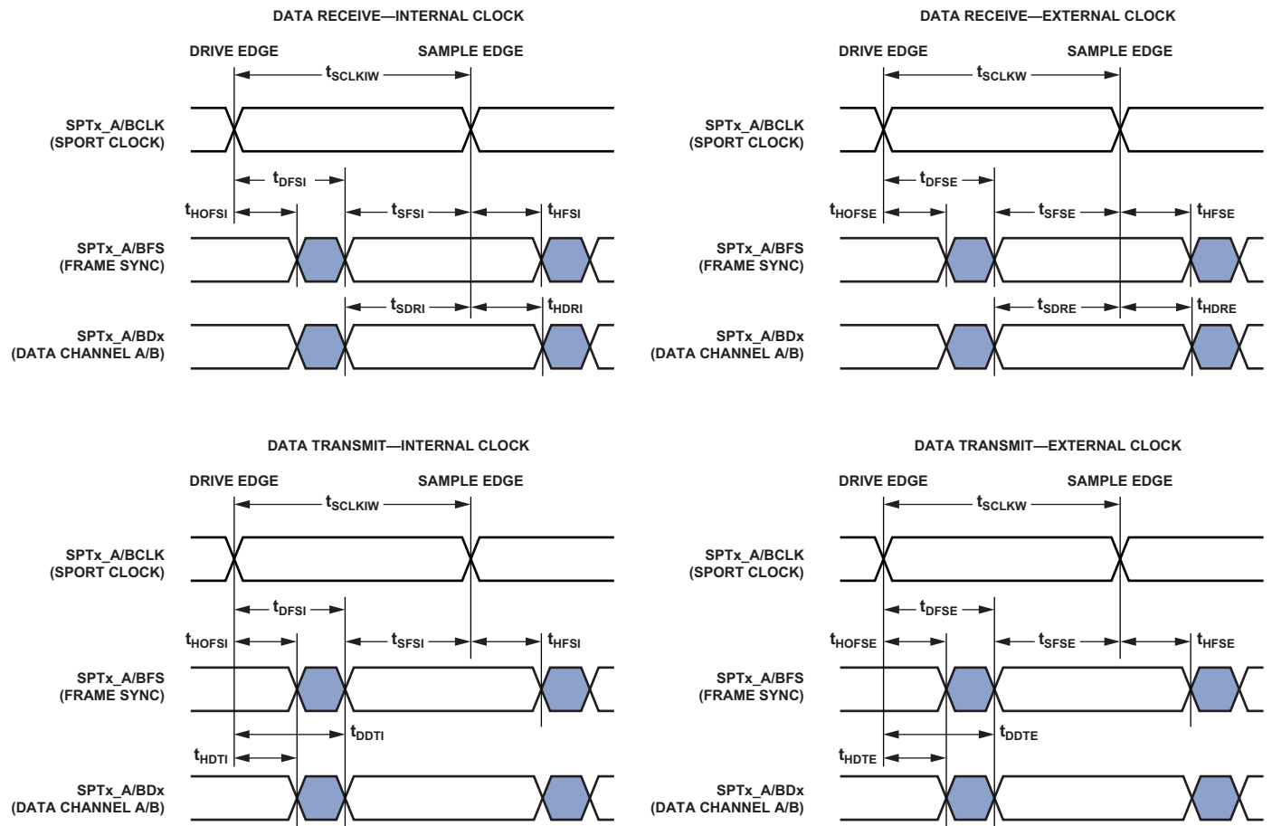
Figure 39. Serial Ports
