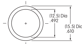
AT537 O-ring Nitrile Butadiene Rubber
