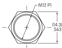
AT503M Hex Face Nut Brass with Chrome Plating
