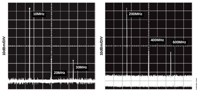
Figure 10. Harmonic Distortion at 10\text{ MHz} and 200\text{ MHz} ; 0\text{ dBm} Input to X (Y) Channels
