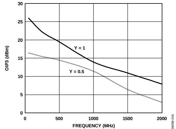
Figure 12. \text{OIP}_3 vs. Frequency Pin 0 dBm, Y = 1\text{ V dc} , 0.5\text{ V dc}
