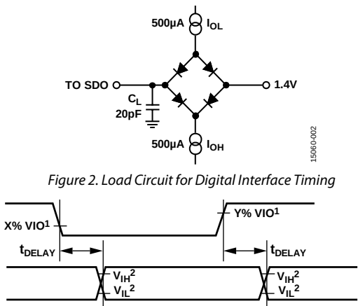
1 FOR VIO ≤ 3.0V, X = 90, AND Y = 10; FOR VIO > 3.0V, X = 70, AND Y = 30. 2 MINIMUM VIH 2 AND MAXIMUM VIL 2 USED. SEE DIGITAL INPUTS SPECIFICATIONS IN TABLE 3 OR TABLE 5.
