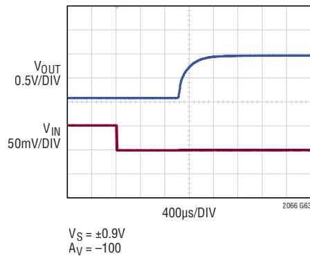
Negative Output Overload Recovery
