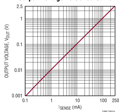
Output Voltage vs Sense Current
