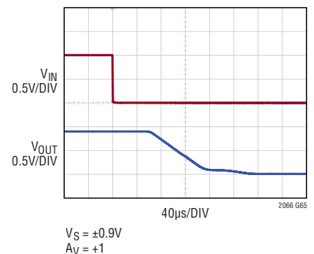
Positive Input Overload Recovery
