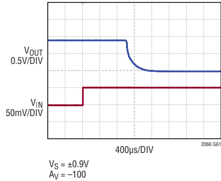
Positive Output Overload Recovery
