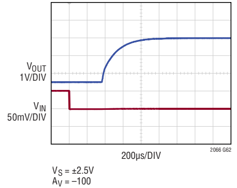
Negative Output Overload Recovery
