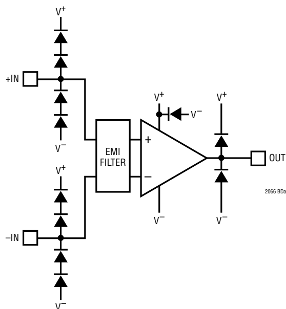
Amplifier
