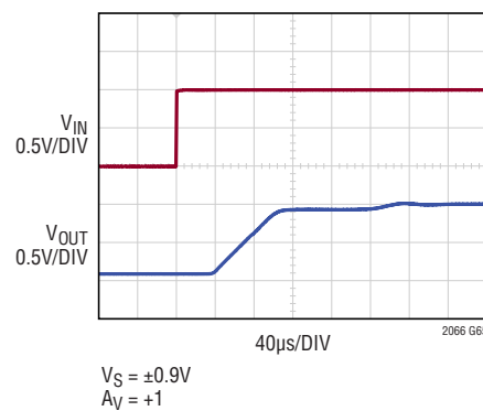
Negative Input Overload Recovery
