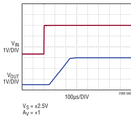
Negative Input Overload Recovery
