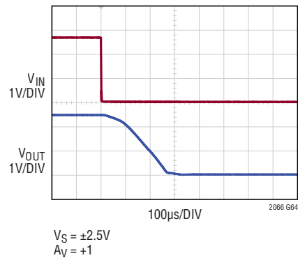
Positive Input Overload Recovery
