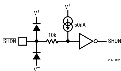
Shutdown Circuit
