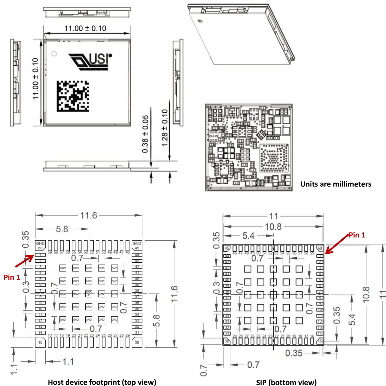
Figure 7: Mechanical Drawings
