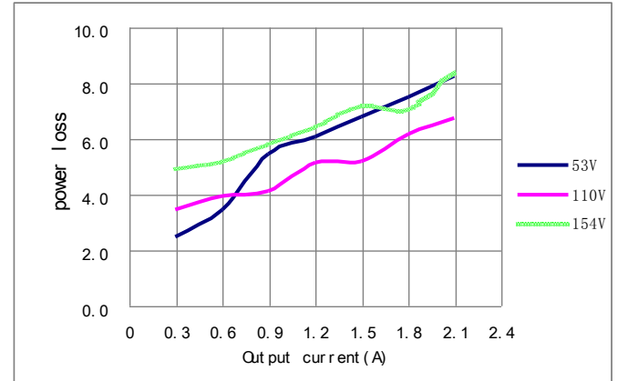
Figure 2: Power dissipation vs. load current for 53, 110 and 154 input voltage at 25°C.
