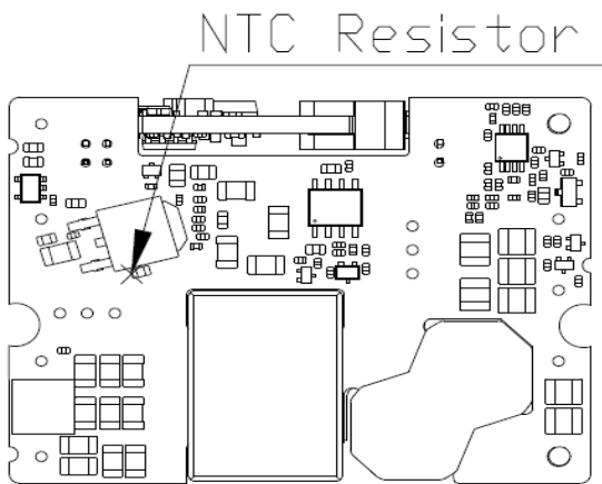
Figure 18: NTC resistor location
