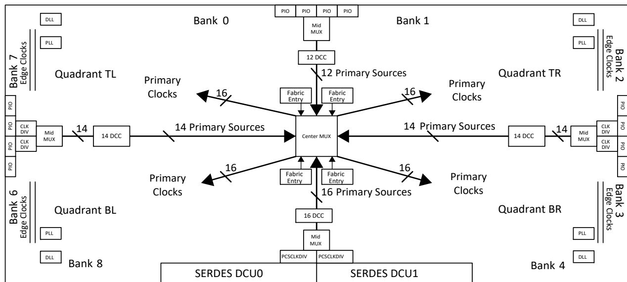
Figure 2.6. LFE5UM/LFE5UM5G-85 Clocking
