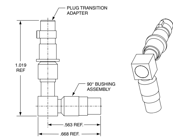
90° Bushing Assembly with Wired Micro D Plug Transition Adapter
