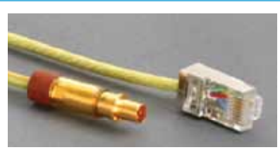
Quadrax Pin with 8P8C "RJ45" Jack
