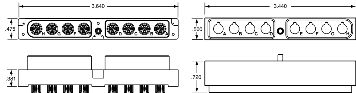
Compliant Pin Quadrax Board Level Connector
