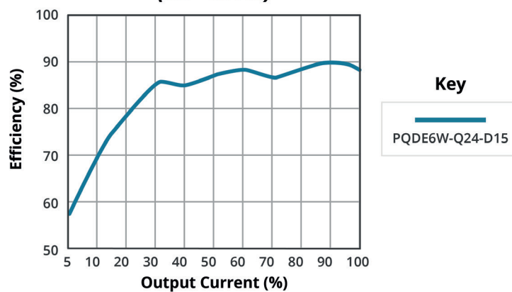
EFFICIENCY VS OUTPUT LOAD (Vin = 48 Vdc)
