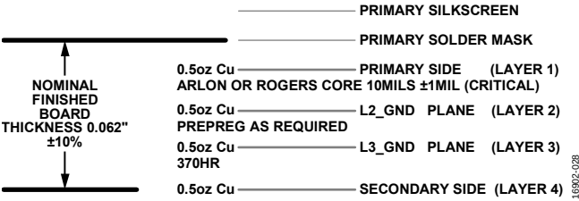
Figure 27. 4-Layer Stackup
