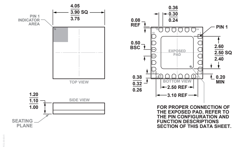
24-Terminal Ceramic Leadless Chip Carrier [LCC] (E-24-2)
