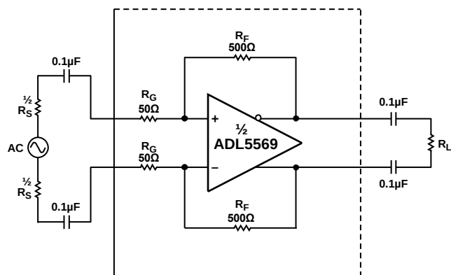
Figure 38. Basic Structure
