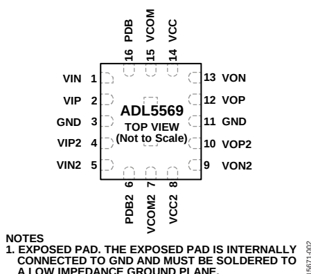
Figure 2. Pin Configuration
