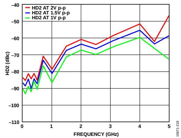
Figure 19. HD2 vs. Frequency for Various Output Voltages Swings
