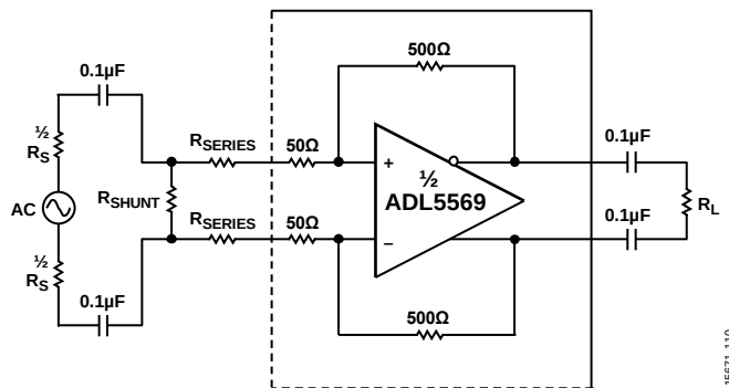
Figure 45. Gain Adjustment Using a Series Resistor
