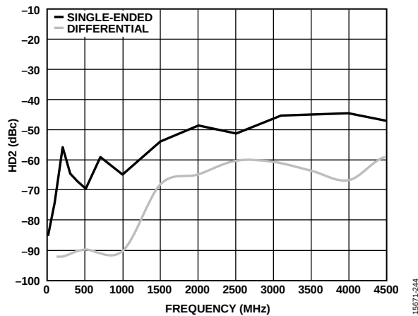
Figure 44. HD2 for Single-Ended and Differential Configurations vs. Frequency, V_{OUT} = 2\text{ V p-p}
