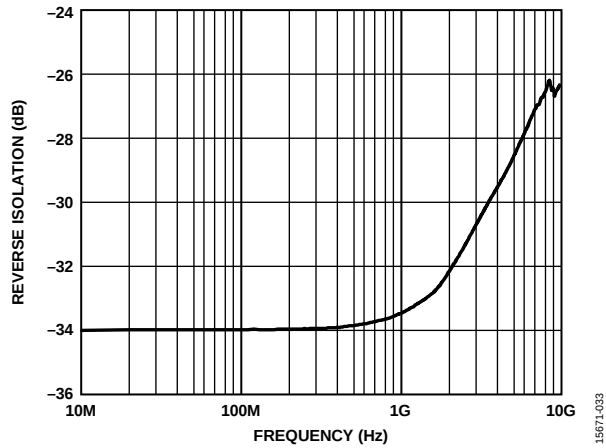
Figure 33. Reverse Isolation (SDD12) vs. Frequency
