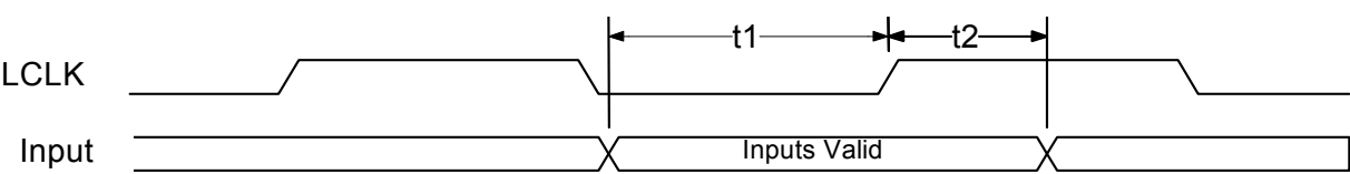
FIGURE 43-17: INPUT TIMING MEASUREMENT CONDITIONS, LPC SIGNALS
