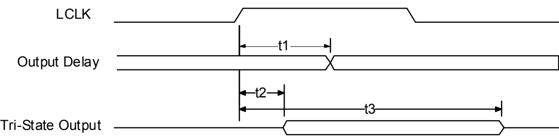
FIGURE 43-16: OUTPUT TIMING MEASUREMENT CONDITIONS, LPC SIGNALS
