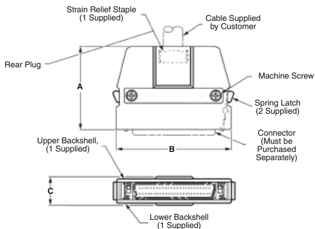
Style A Straight Exit with Latches
