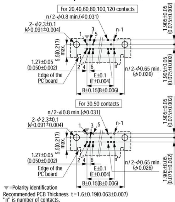
Printed Circuit Board Layout (Component Side View)
