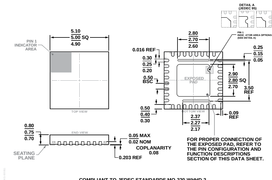
Figure 40. 32-Lead Lead Frame Chip Scale Package [LFCSP] 5 mm × 5 mm Body and 0.75 mm Package Height (CP-32-31) Dimensions shown in millimeters
