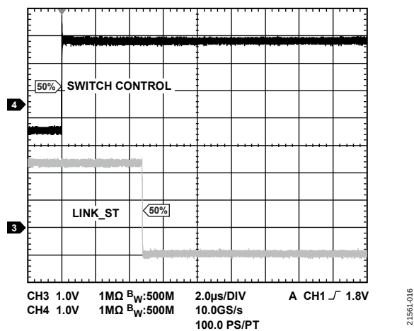
Figure 17. Enhanced Link Detection 100 Mbps, 100 m Cable with Single Wire Break
