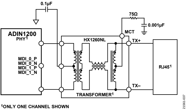
1ONLY ONE CHANNEL SHOWN Figure 34. Isolation Using Discrete Magnetics, Only One Channel Shown, Each Channel has Separate Components to Ground
