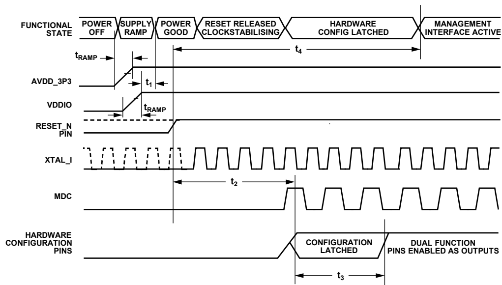
Figure 2. Power-Up Timing
