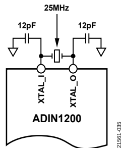
Figure 32. Crystal Oscillator Connection
