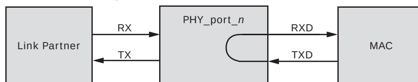
Figure 18 • Near-End Loopback Diagram
